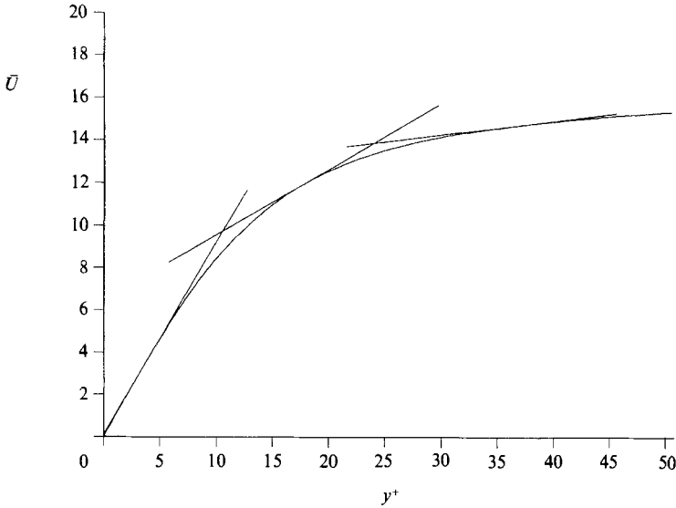
FIGURE 6. Mean velocity profile in channel flow showing the suitability of linear approximations.
