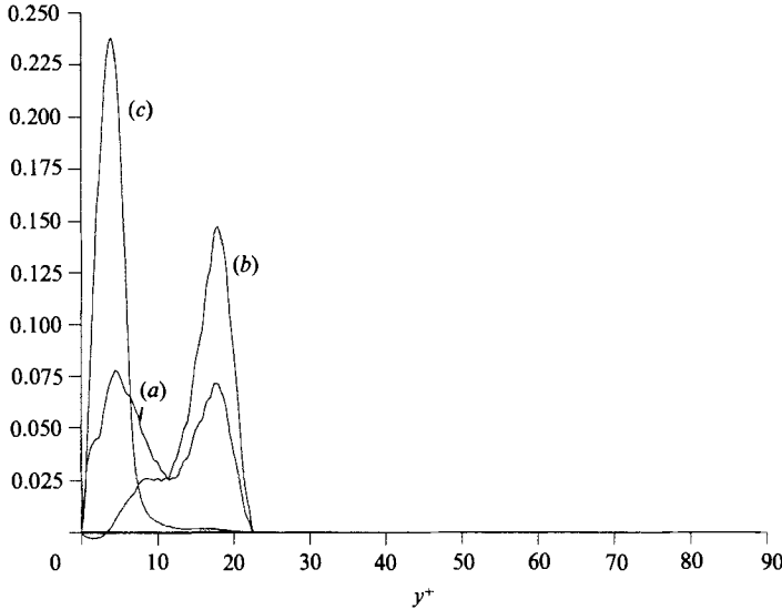
FIGURE 7. Computed probability density functions at y^+ = 3.8 : (a) gradient term; (b) \Phi_2 ; (c) initial positions of particles.
