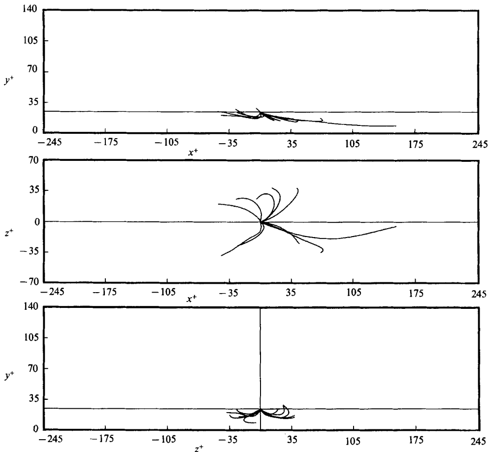
FIGURE 13. Visualizations of particle trajectories. Ten paths contributing most negatively to \overline{v_a(U_a - U_b)} at y^+ = 24.6 .
