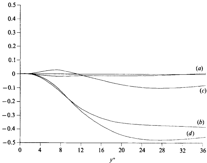
FIGURE 15. Spatial dependence of terms in Reynolds stress decomposition (7): (a) \overline{u_b v_a} ; (b) v_a(\overline{U_b} - \overline{U_a}) ; (c) v_a(\overline{U_a} - \overline{U_b}) ; (d) \overline{w w} .
