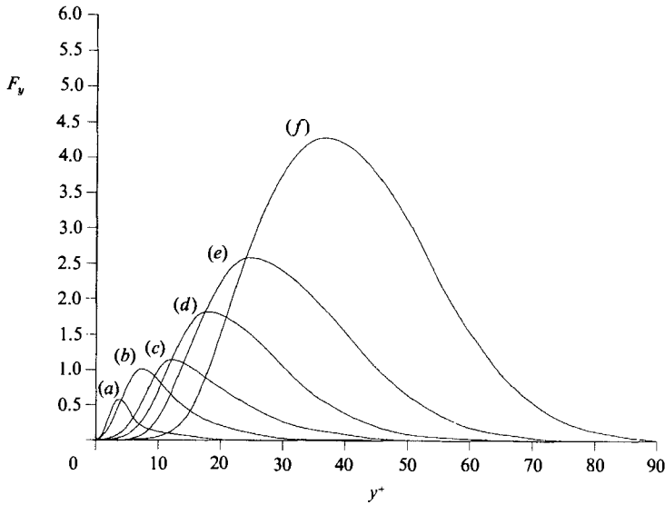
FIGURE 17. The function F_y(r) at each y -position: (a-f) correspond to y^+ = 3.8, 7.3, 12.0, 17.8, 24.6 and 36.6 , respectively.
