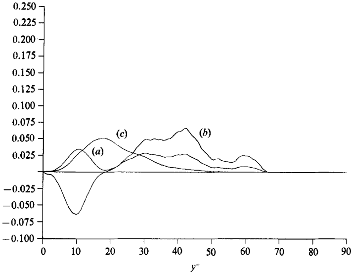
FIGURE 8. Computed probability density functions at y^+ = 17.8 : (a) gradient term; (b) \Phi_2 ; (c) initial positions of particles.
