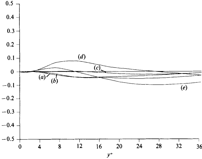
FIGURE 12. Quadrant decomposition of term \Phi_1 in (3): (a) Q1; (b) Q2; (c) Q3; (d) Q4; (e) total.
