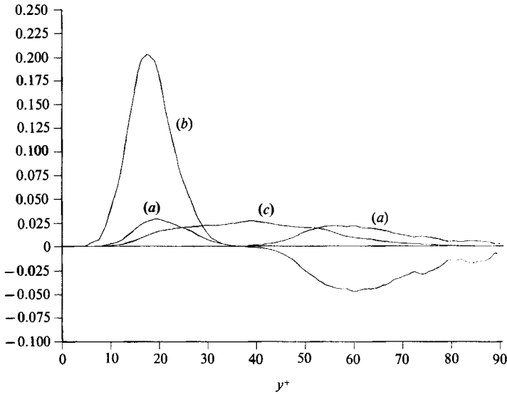
FIGURE 9. Computed probability density functions at y^+ = 36.6 : (a) gradient term; (b) \Phi_2 ; (c) initial positions of particles.
