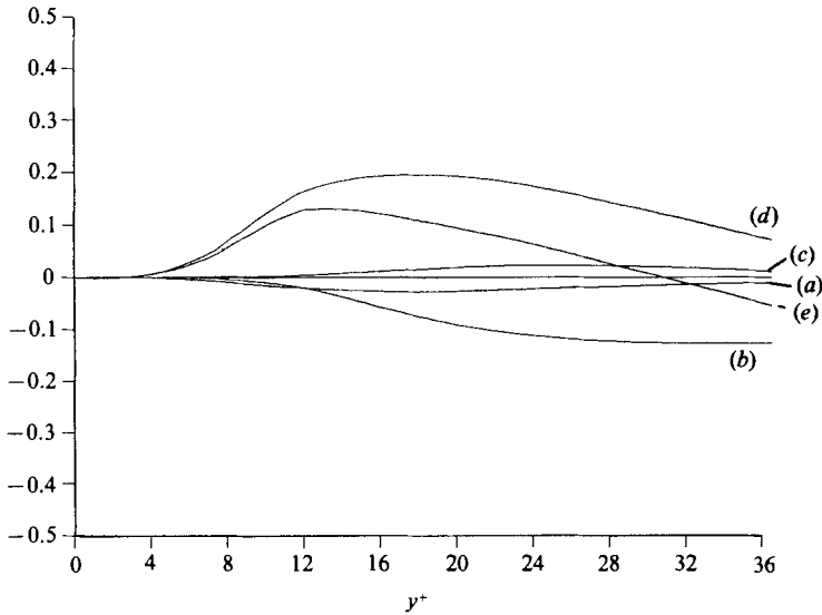
FIGURE 11. Quadrant decomposition of term \Phi_2 in (3): (a) Q1; (b) Q2; (c) Q3; (d) Q4; (e) total.
