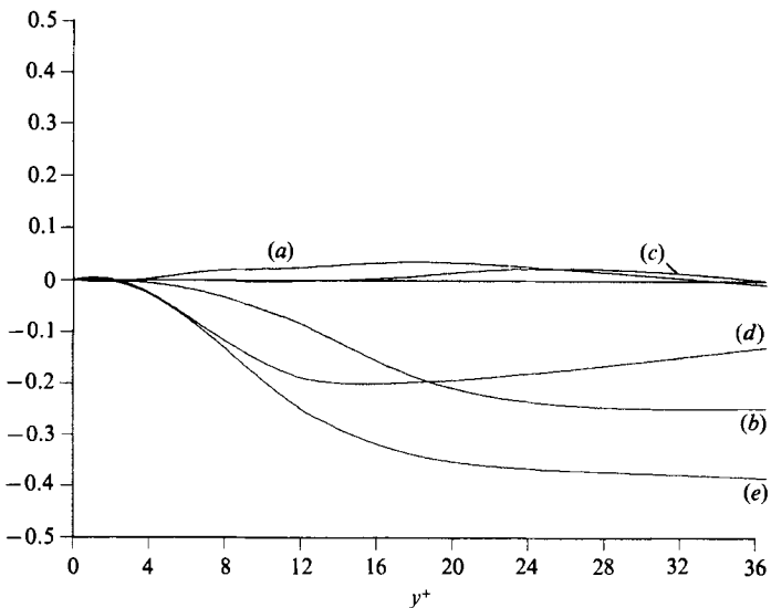
FIGURE 16. Quadrant decomposition of \overline{v_a(\overline{U_b} - \overline{U_a})} in (7): (a) Q1; (b) Q2; (c) Q3; (d) Q4; (e) total.
