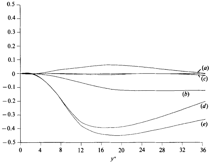
FIGURE 10. Quadrant decomposition of the gradient term in (3): (a) Q1; (b) Q2; (c) Q3; (d) Q4; (e) total.
