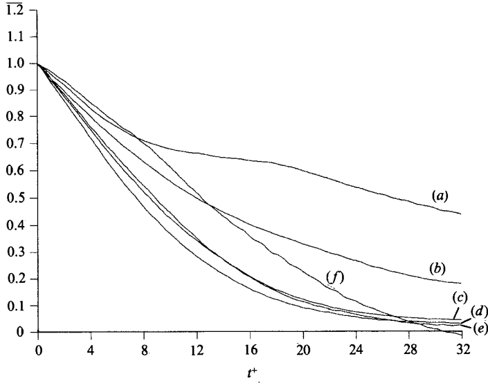
FIGURE 2. Time development of \overline{u_b v_a} correlation for each ensemble of paths: (a-f) correspond to y^+ = 3.8, 7.3, 12.0, 17.8, 24.6 and 36.6 , respectively.
