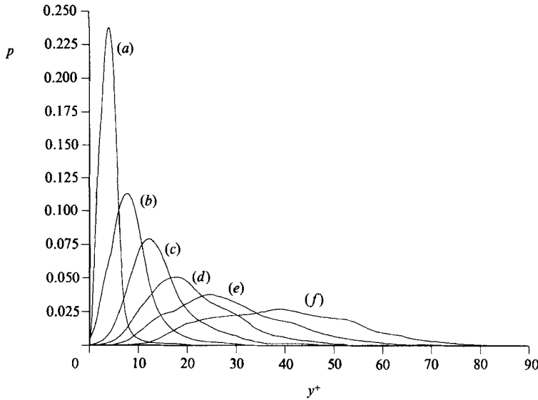
FIGURE 4. Probability density functions of initial particle positions: (a-f) correspond to y^+ = 3.8, 7.3, 12.0, 17.8, 24.6 and 36.6 , respectively.
