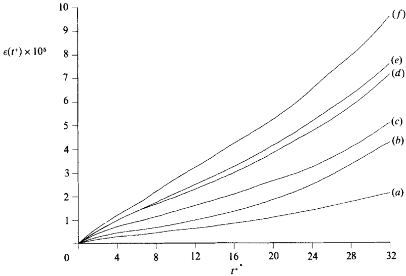
FIGURE 1. Root-mean-square positional errors for computed particle paths: (a-f) correspond to y^+ = 3.8, 7.3, 12.0, 17.8, 24.6 and 36.6 , respectively.
