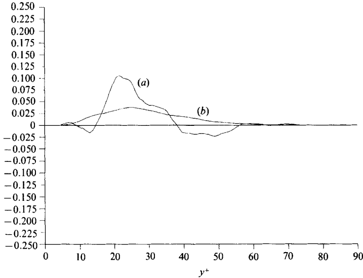
FIGURE 14. Computed probability density functions at y^+ = 24.6 : (a) \Phi_1 ; (b) initial positions of particles.
